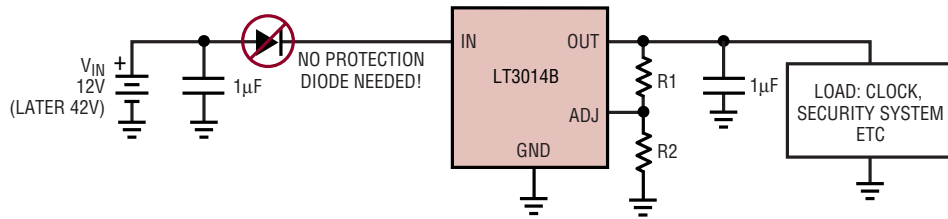
LT3014B Automotive Application
