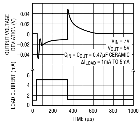
Transient Response
