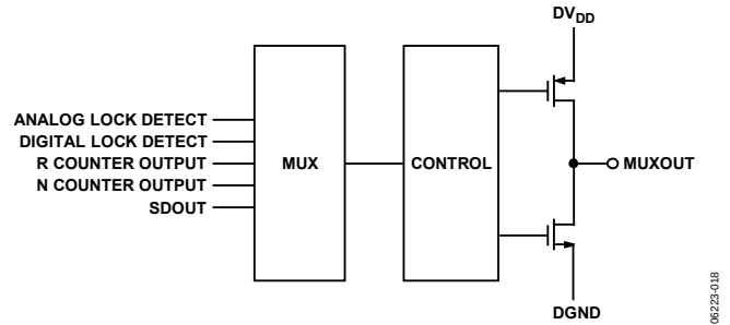
Figure 18. MUXOUT Circuit
