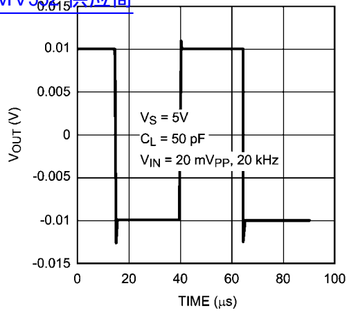
Small Signal Transient Response
