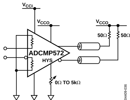
Figure 28. Adding Hysteresis Using the HYS Control Pin
