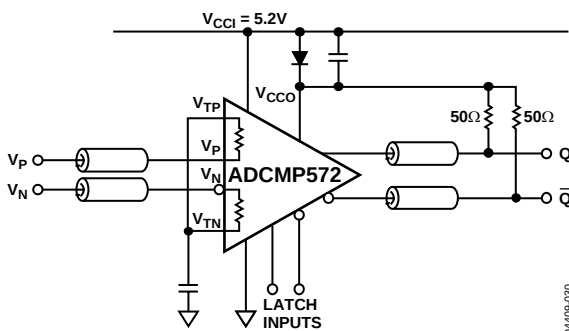
Figure 22. LVDS to 50 Ω Back Terminated RSPECL Receiver
