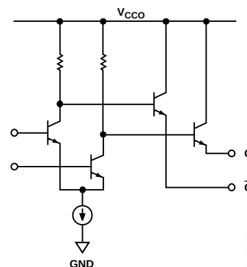
Figure 16. Simplified Schematic Diagram of the ADCMP573 RSPECL Output Stage
