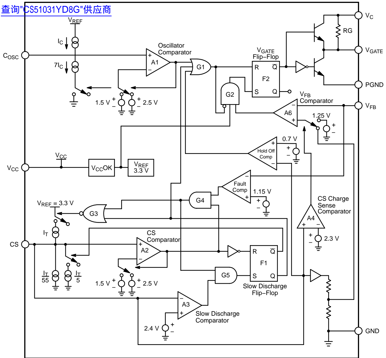
Figure 2. Block Diagram
