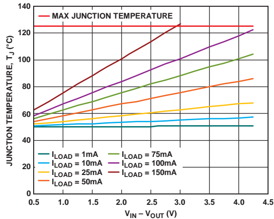
Figure 38. TSOT, 0 mm 2 of PCB Copper, T A = 50°C
