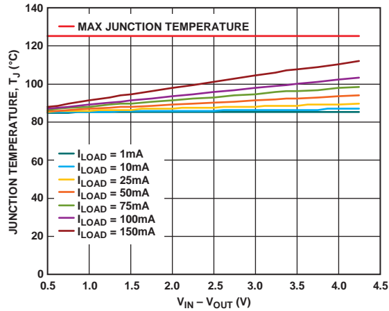
Figure 39. TSOT, 100 mm 2 of PCB Copper, Board Temperature = 85°C
