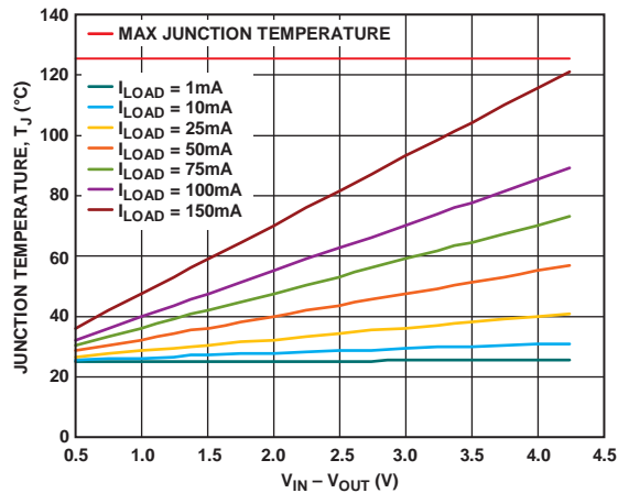
Figure 40. WLCSF, 500 mm 2 of PCB Copper, T A = 25°C
