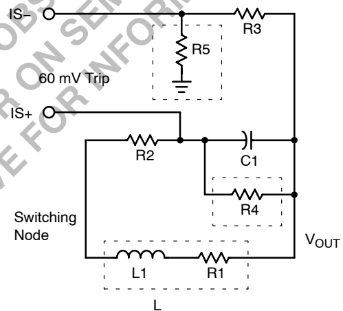
Figure 8. Current Limit
