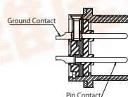
Receptacle Connector
