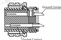
Plug Connector
