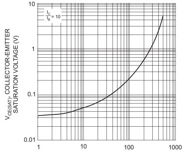
Fig. 8, Typical Collector-Emitter Saturation Voltage vs. Collector Current (PNP-3906)
