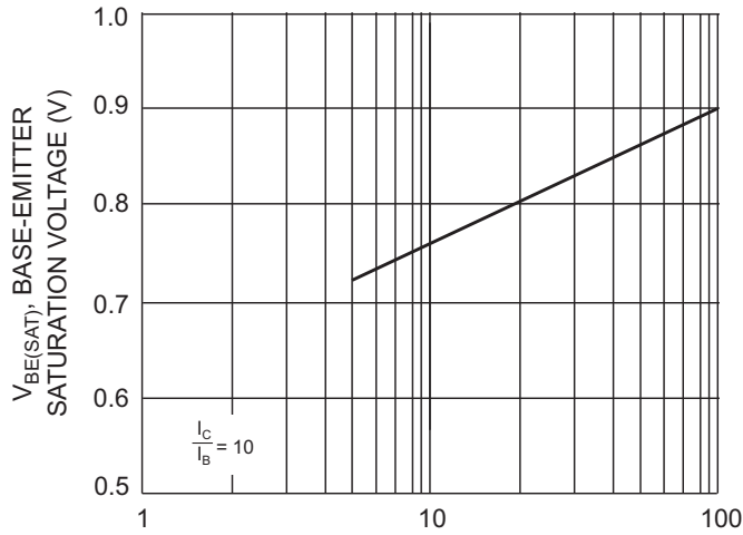
Fig. 9, Typical Base-Emitter Saturation Voltage vs. Collector Current (PNP-3906)
