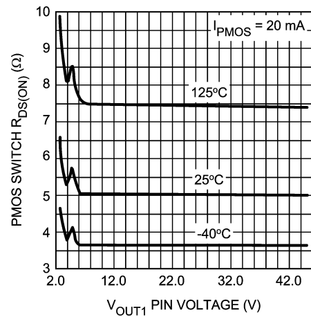
PMOS R DS(ON) (Figure 2: P1) vs V IN
