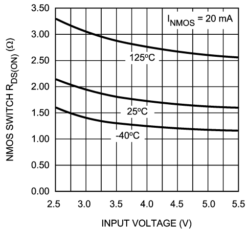
NMOS R DS(ON) (Figure 2: N2) vs V IN
