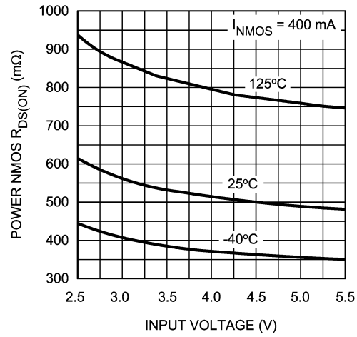
Power NMOS R DS(ON) (Figure 2: N1) vs V IN
