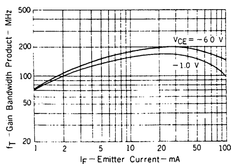
GAIN BANDWIDTH PRODUCT vs. EMITTER CURRENT
