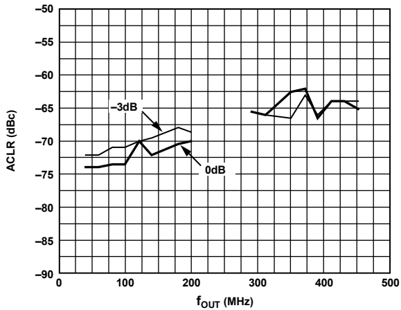
Figure 36. AD9783 ACLR for Second Adjacent Channel Four-Carrier W-CDMA Over Digital Input Level Baseband and Mix Modes, at 491.52 MSPS, FS = 20 mA
