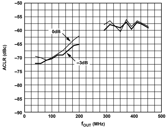
Figure 35. AD9783 ACLR for First Adjacent Channel Four-Carrier W-CDMA Over Digital Input Level Baseband and Mix Modes, at 491.52 MSPS, FS = 20 mA
