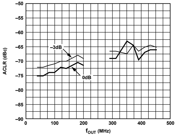
Figure 37. AD9783 ACLR for Third Adjacent Channel Four-Carrier W-CDMA Over Digital Input Level Baseband and Mix Modes, at 491.52 MSPS, FS = 20 mA
