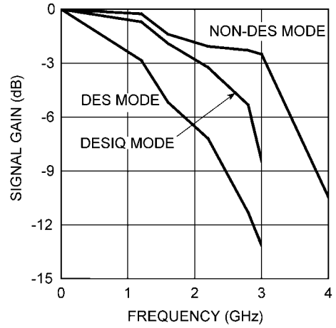
FULL POWER BANDWIDTH (ADC10D1500)
