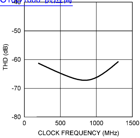
THD vs. CLOCK FREQUENCY (ADC10D1000) 查询"ADC10D1000"供应商
