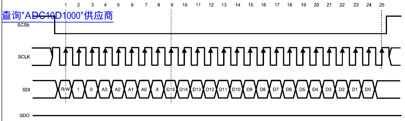
FIGURE 13. Serial Data Protocol - Write Operation
