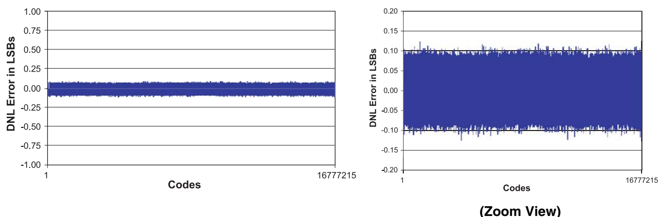
Figure 10. CS5566 DNL Plot
