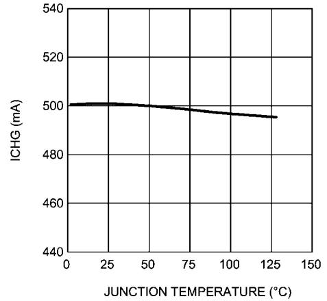
IC CHG vs. Temperature CHG_DET = 5V, VBATT = 3.75V, CC
