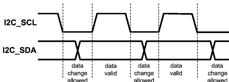
I 2 C Signals: Data Validity
