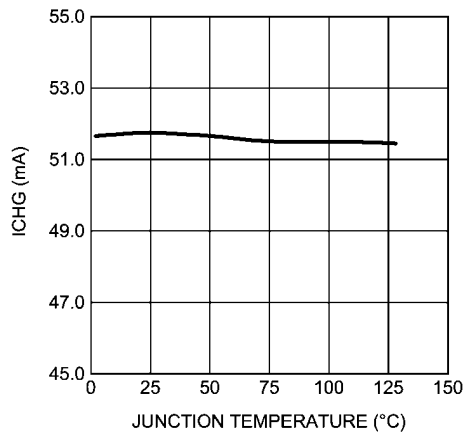
IC CHG vs. Temperature CHG_DET = 5V, VBATT = 2.5V, Prequal
