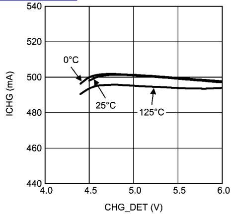
IC CHG vs. CHG_DET VBATT = 3.5V, CC
