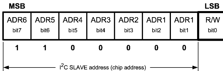
I 2 C Chip Address
