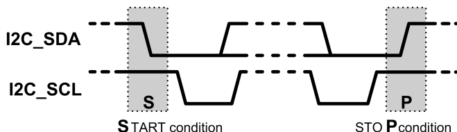
START and STOP Conditions
