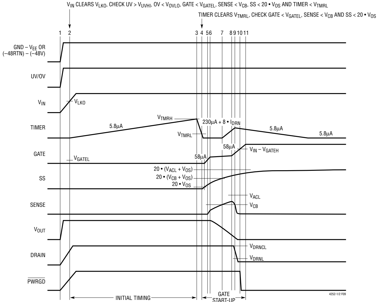
Figure 9. System Power-Up Timing (All Waveforms are Referenced to V_{EE} )
