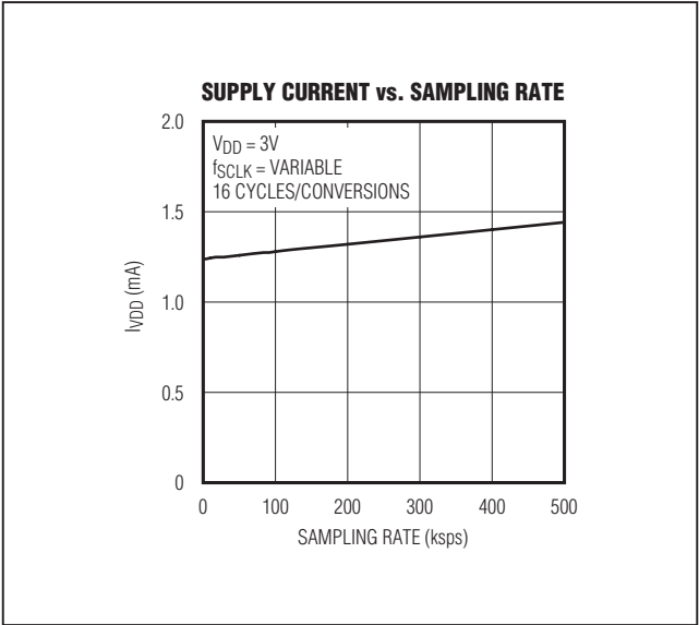
Figure 11. Supply Current vs. Sample Rate (Normal Operating Mode, 3Msps Devices)
