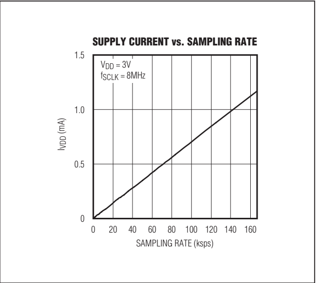
Figure 12. Supply Current vs. Sample Rate (Device Powered Down Between Conversions, 3Msps Devices)
