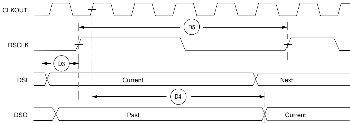
Figure 21. BDM Serial Port AC Timing
