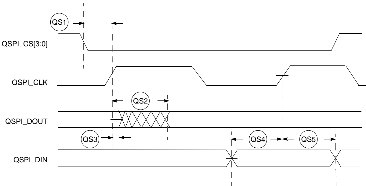
Figure 15. QSPI Timing
