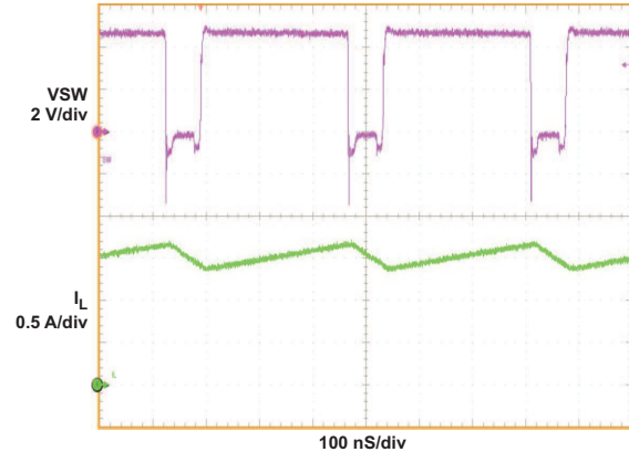
Figure 6. VBUS = 5 V, VBAT = 2.6 V, Voreg = 4.2 V, Ichg = 1550 mA
