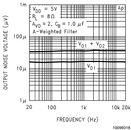
Noise Floor
