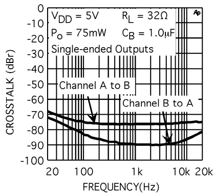
Channel Separation
