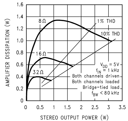
LM4873IBL Stereo Output Power vs Power Dissipation
