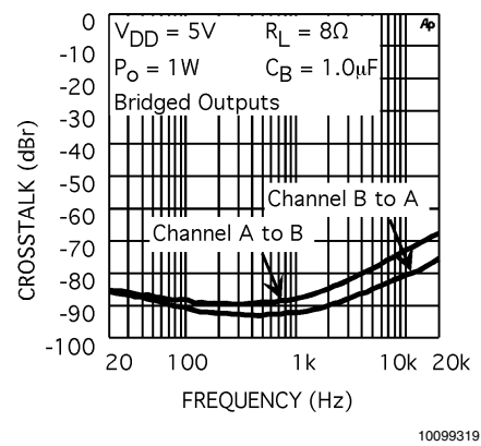
Channel Separation
