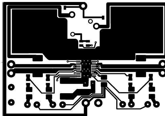
FIGURE 5. Recommended MTE PC Board Layout: Component-Side Layout
