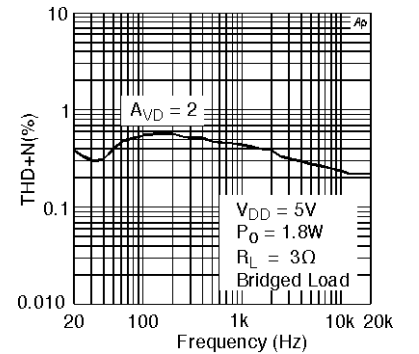
LM4873MTE, LM4873LQ THD+N vs Frequency
