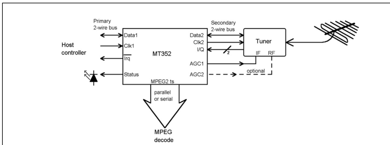
Figure 5 - Primary Interfaces
