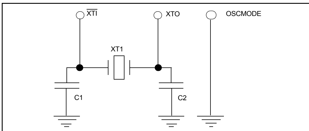
Figure 11 - Crystal Oscillator Circuit
