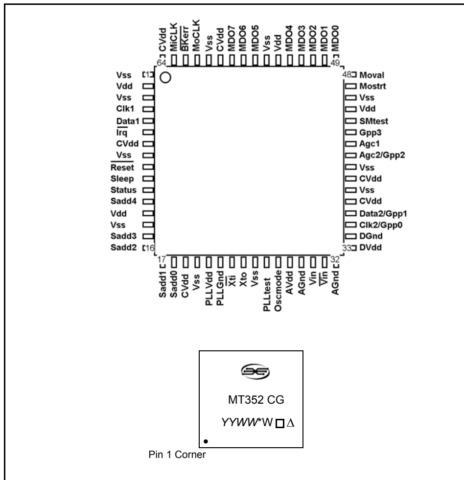
Figure 2 - Package Outline
