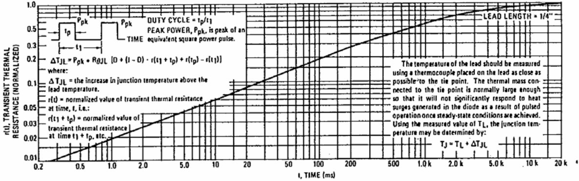
FIGURE 5 -- THERMAL RESPONSE
