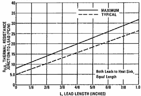
FIGURE 4 - STEADY-STATE THERMAL RESISTANCE
