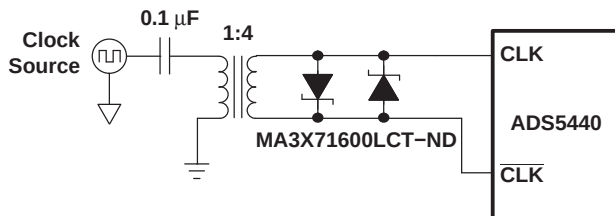
Figure 40. Differential Clock
