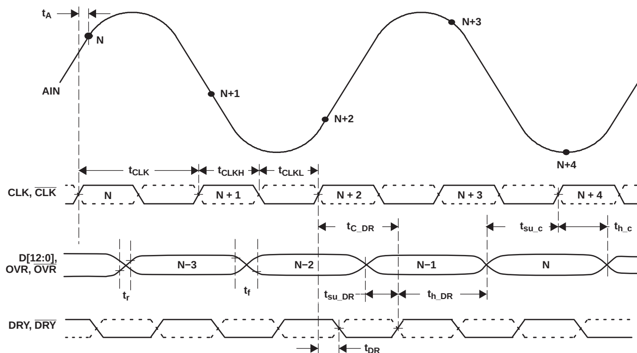
Figure 2. Timing Diagram
