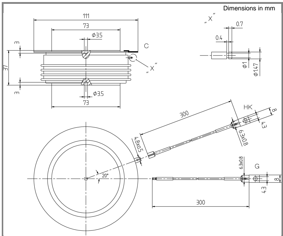
Case B 20 (JEDEC: TO-200AF)
