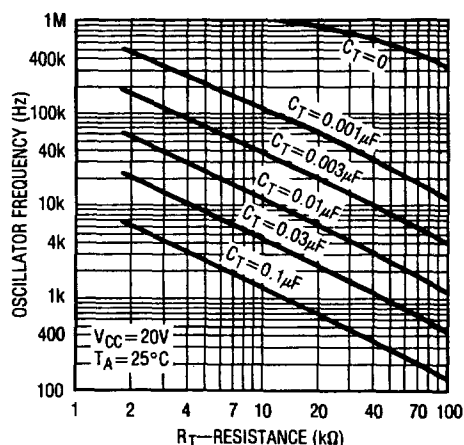
Oscillator Frequency vs Timing Resistance
