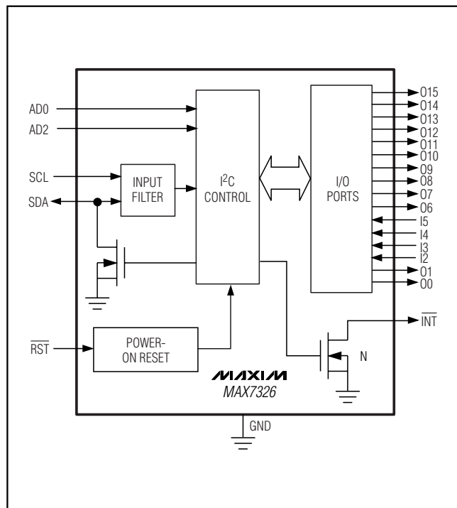
Functional Diagram
