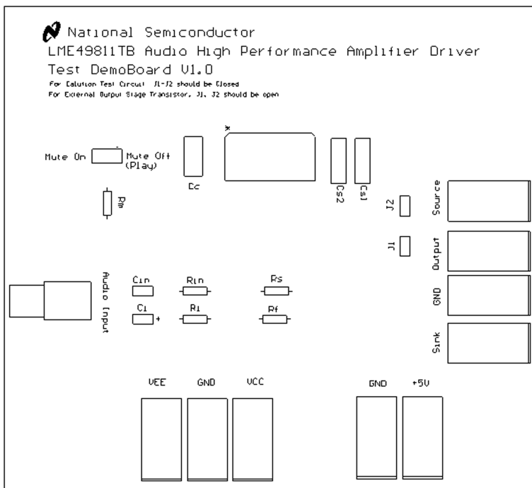
Silkscreen Layer
