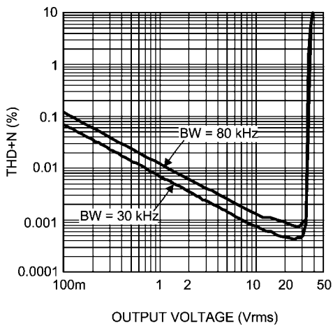
THD+N vs Output Voltage +V_{CC} = -V_{EE} = 50V, f = 1kHz
