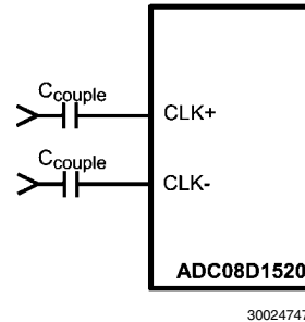
FIGURE 14. Differential (LVDS) Input Clock Connection
