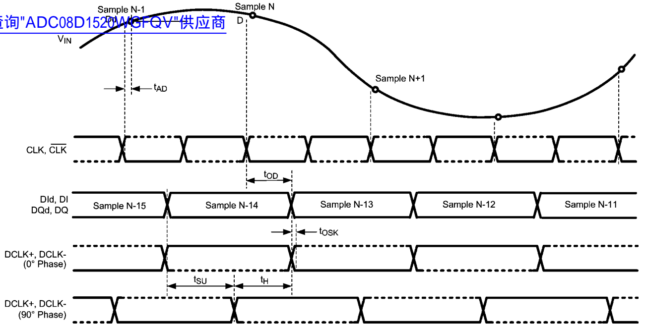
FIGURE 5. DDR Clcking in Non-Demultiplexed and Non-DES Mode
