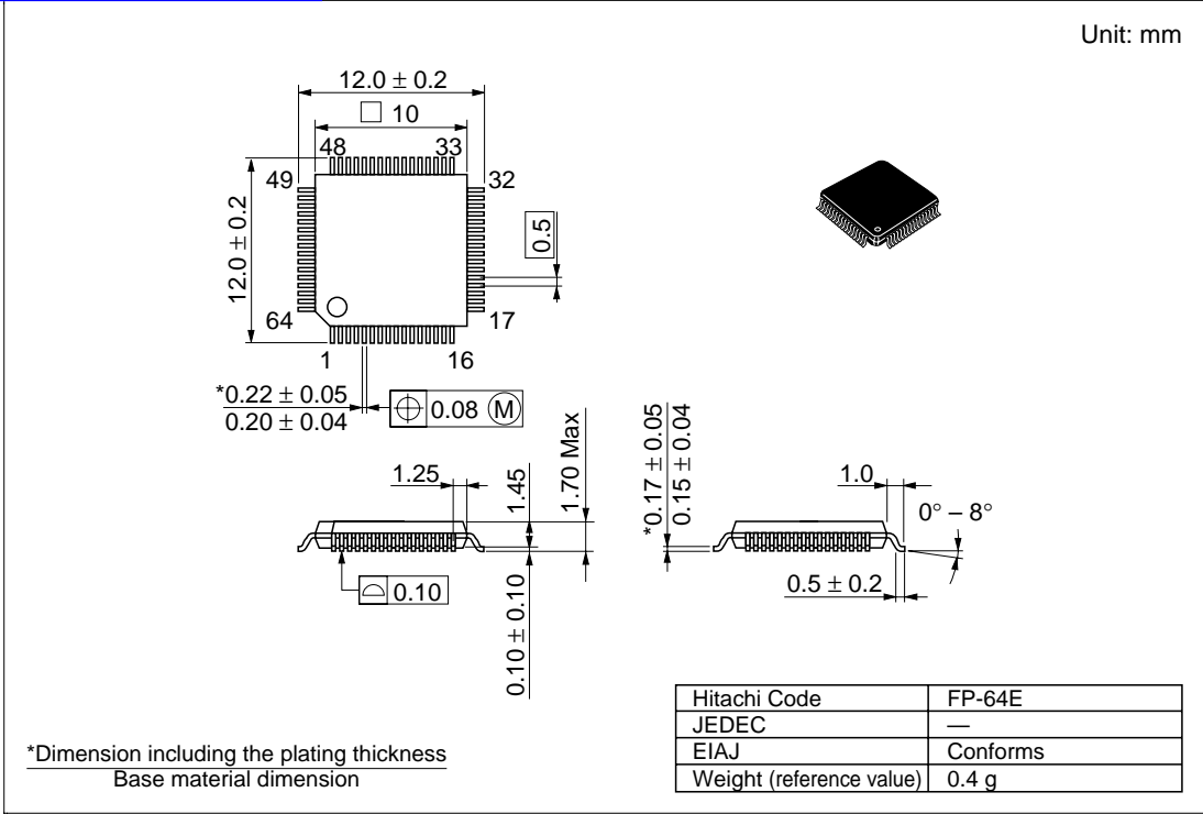
Figure F.2 FP-64E Package Dimensions
