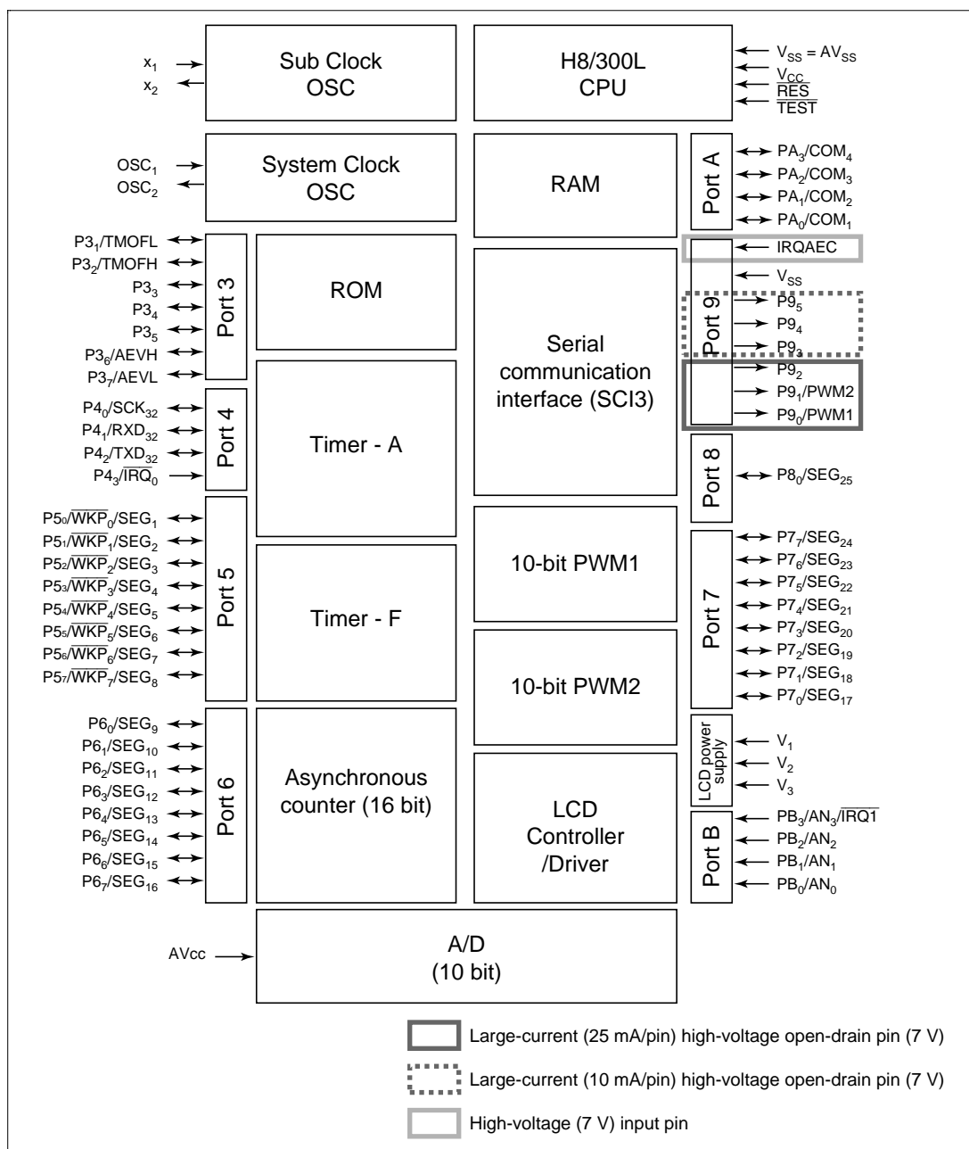
Figure 1.1 Block Diagram
