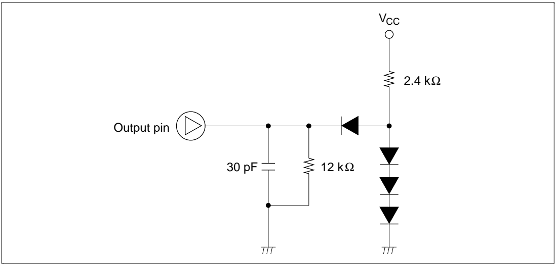
Figure 14.6 Output Load Condition
