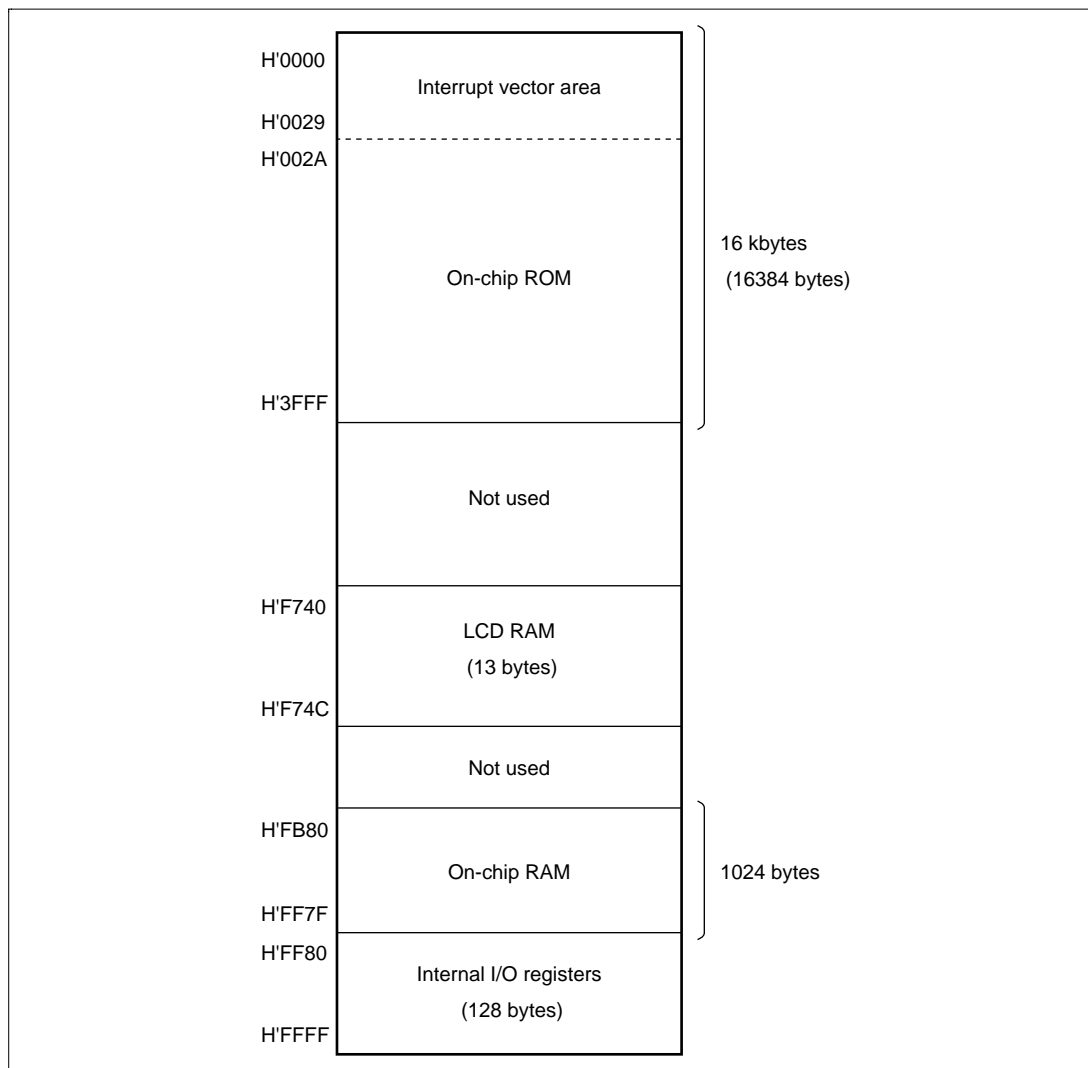
Figure 2.16 (1) H8/3802 Memory Map
