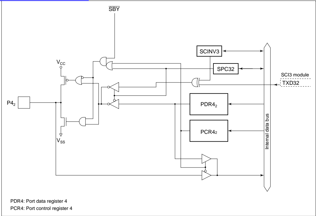
Figure C.2 (b) Port 4 Block Diagram (Pin P4 2 )
