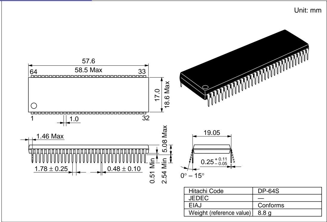
Figure F.3 DP-64S Package Dimensions
