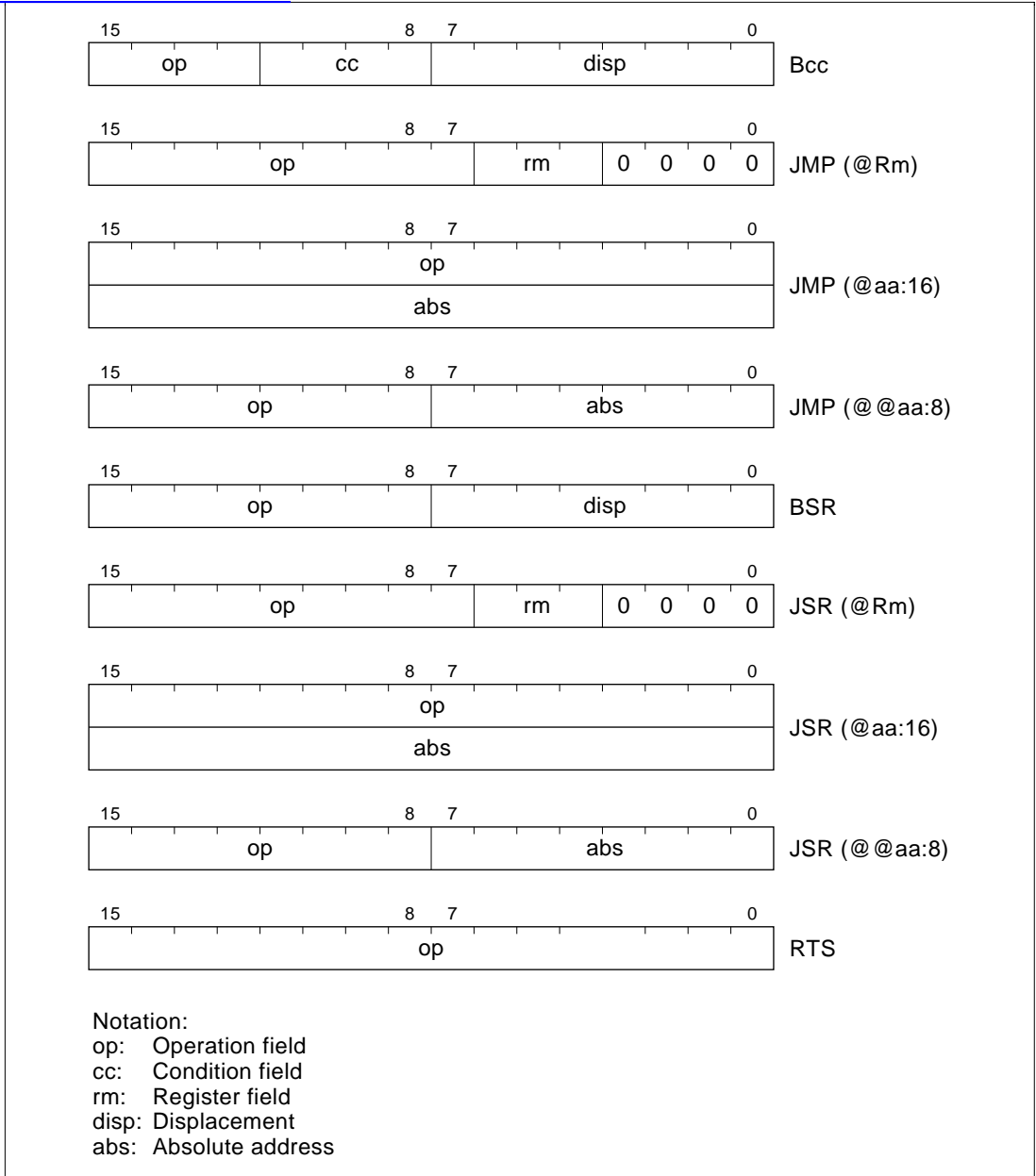
Figure 2.8 Branching Instruction Codes
