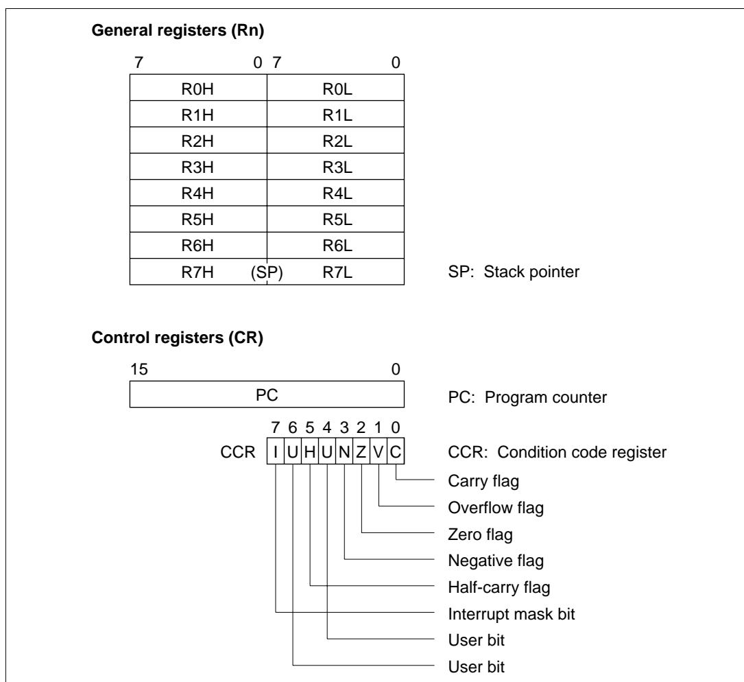
Figure 2.1 CPU Registers
