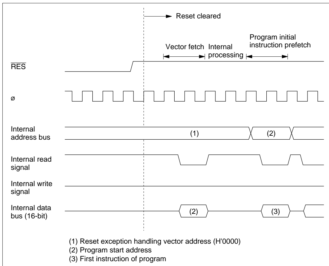
Figure 3.1 Reset Sequence
