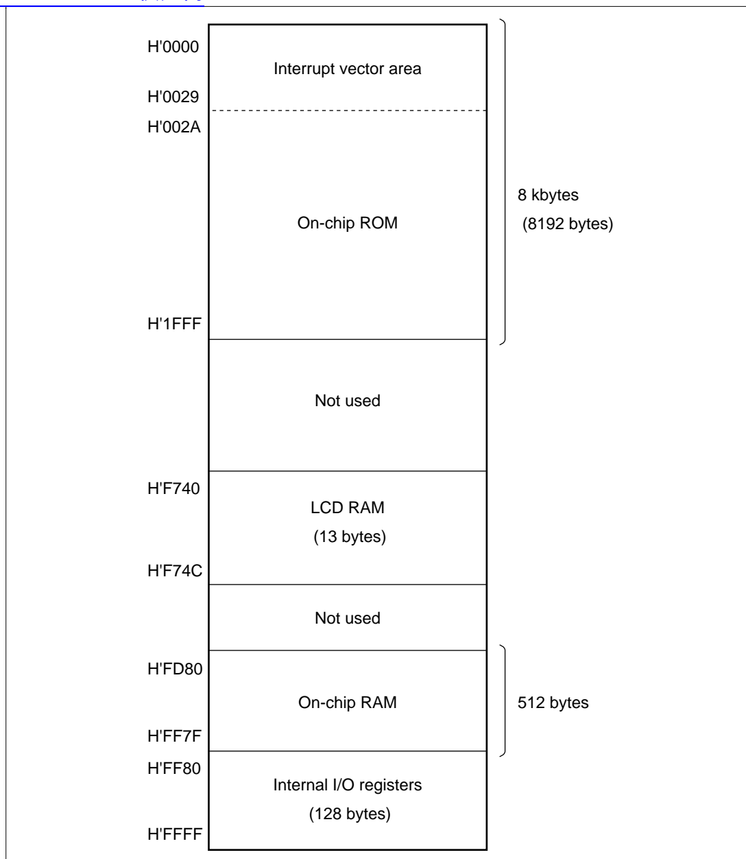
Figure 2.16 (3) H8/3800 Memory Map
