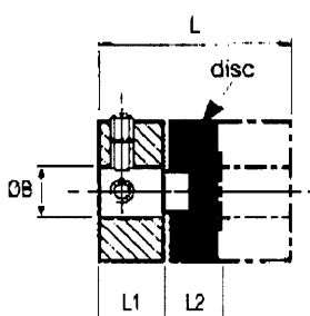
Refs. 450, 454 Set screw style
