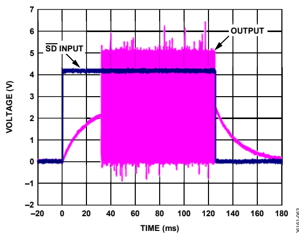
Figure 42. Turn-Off Response
