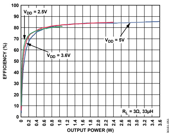
Figure 28. Efficiency vs. Output Power into 3 \Omega
