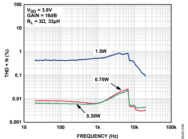
Figure 14. THD + N vs. Frequency, V_{DD} = 3.6\text{ V} , R_L = 3\ \Omega , A_V = 18\text{ dB}
