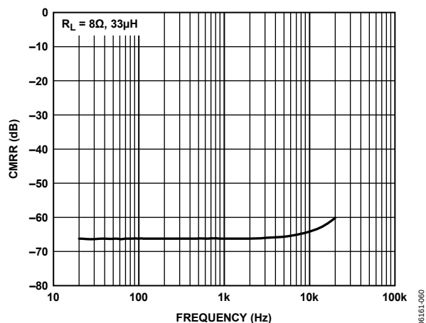
Figure 39. Common-Mode Rejection Ratio vs. Frequency
