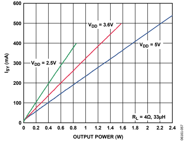
Figure 36. Supply Current vs. Output Power into 4 \Omega
