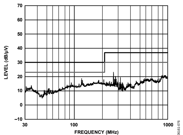
Figure 47. EMI Emissions from SSM2311
