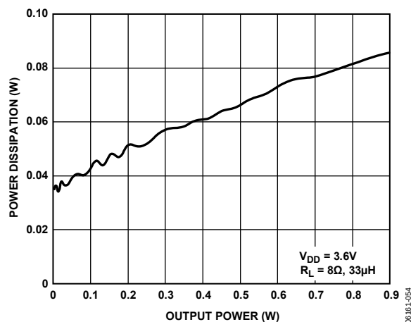
Figure 32. Power Dissipation vs. Output Power into 8 \Omega at V_{DD} = 3.6 V
