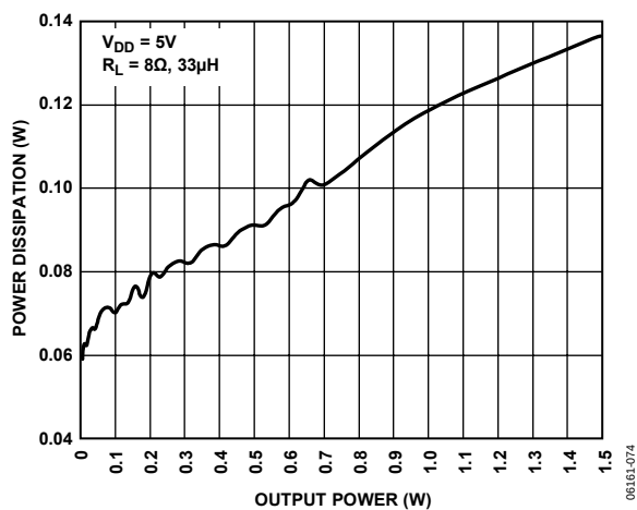
Figure 29. Power Dissipation vs. Output Power into 8 \Omega at V_{DD} = 5.0 V
