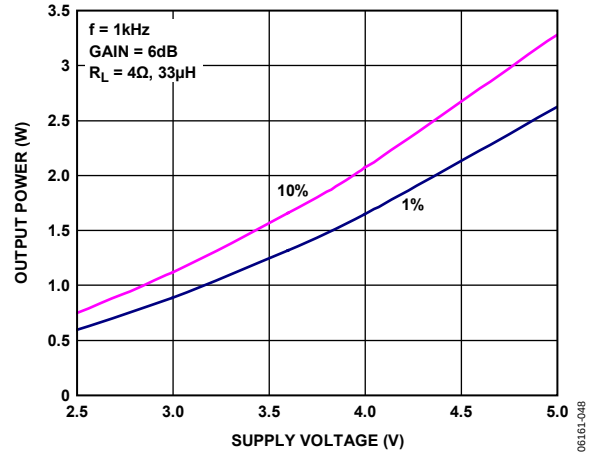
Figure 24. Maximum Output Power vs. Supply Voltage, R_L = 4\ \Omega , A_v = 6\ \text{dB}
