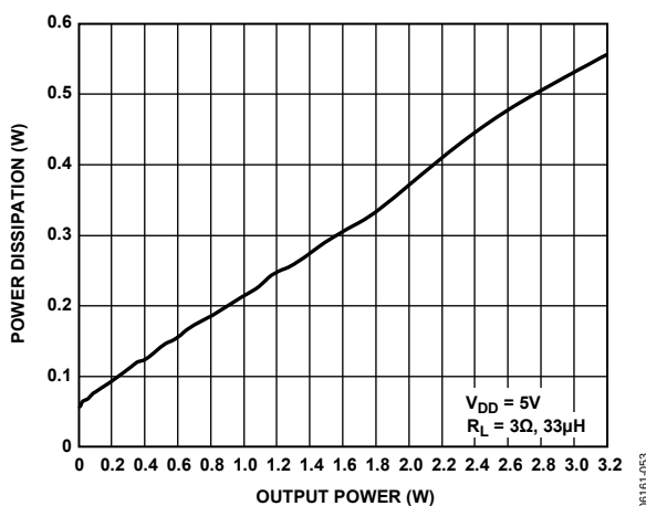
Figure 31. Power Dissipation vs. Output Power into 3 \Omega at V_{DD} = 5.0 V
