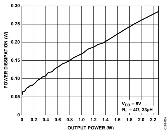
Figure 30. Power Dissipation vs. Output Power into 4 \Omega at V_{DD} = 5.0 V
