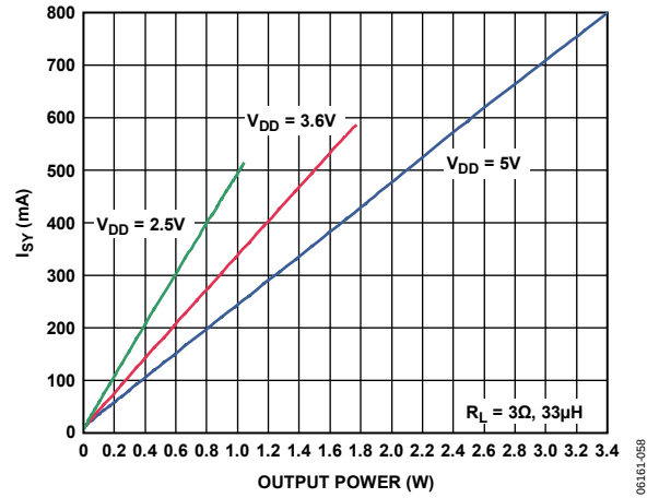
Figure 37. Supply Current vs. Output Power into 3 \Omega
