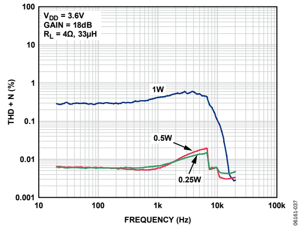
Figure 13. THD + N vs. Frequency, V_{DD} = 3.6\text{ V} , R_L = 4\ \Omega , A_V = 18\text{ dB}
