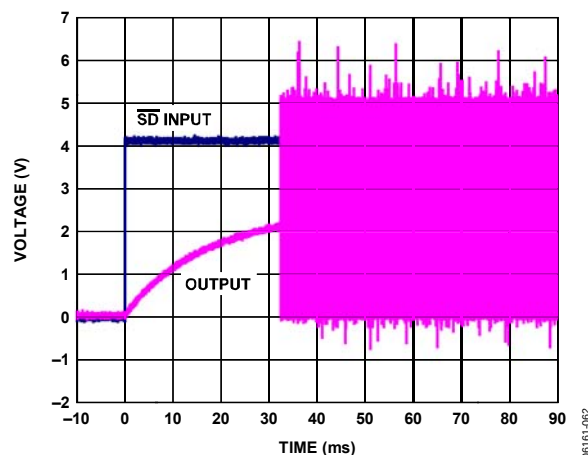
Figure 41. Turn-On Response
