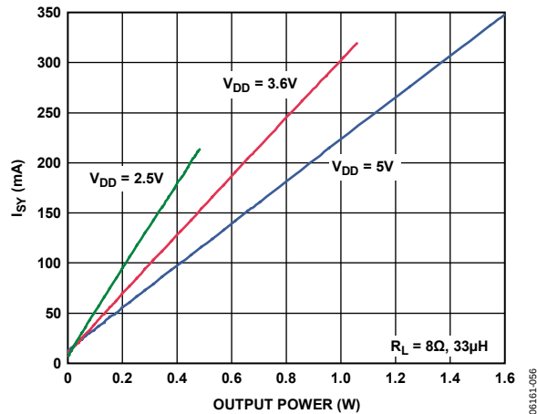
Figure 35. Supply Current vs. Output Power into 8 \Omega
