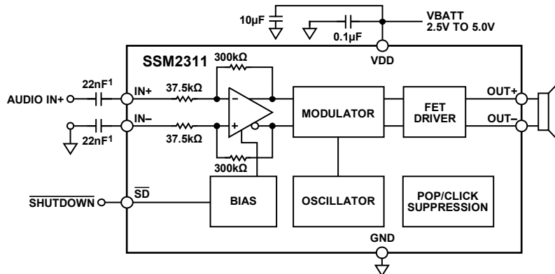
Figure 44. Single-Ended Input Configuration
