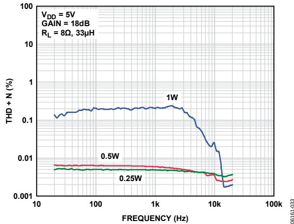
Figure 9. THD + N vs. Frequency, V_{DD} = 5.0\text{ V} , R_L = 8\ \Omega , A_V = 18\text{ dB}
