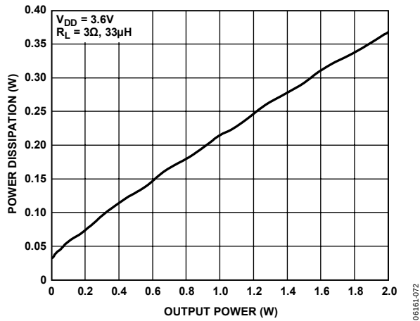
Figure 34. Power Dissipation vs. Output Power into 3 \Omega at V_{DD} = 3.6V
