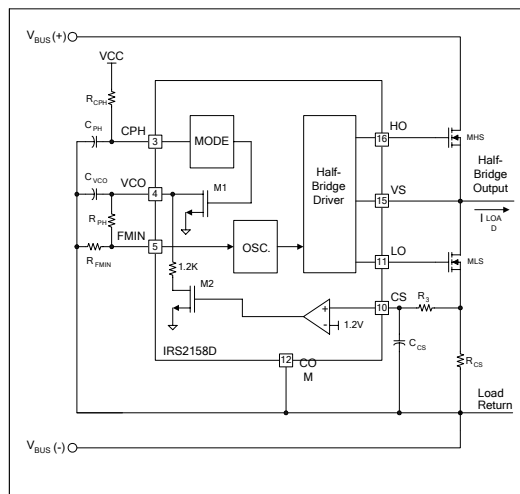
Figure 5: Ignition circuitry.
