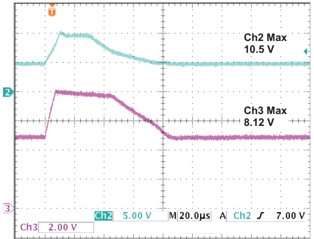
Figure 4. OVP Response for Input Step, V_{IN} = 5\text{ V to }10\text{ V} back to 5\text{ V} , t_r = 10\mu\text{s} , CH2 input voltage peak = 10.5\text{ V} , CH3 output voltage peak = 8.12\text{ V} . OVP duration is shorter than Blanking time.
