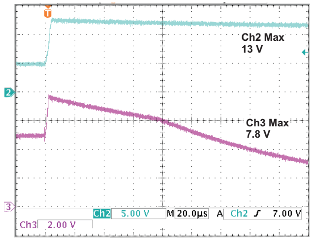
Figure 5. OVP Response for Input Step, V_{IN} = 5\text{ V to }12\text{ V} , t_r = 4\mu\text{s} . CH2 input voltage peak = 13\text{ V} , CH3 output voltage peak = 7.8\text{ V} . OVP duration is longer than Blanking time.
