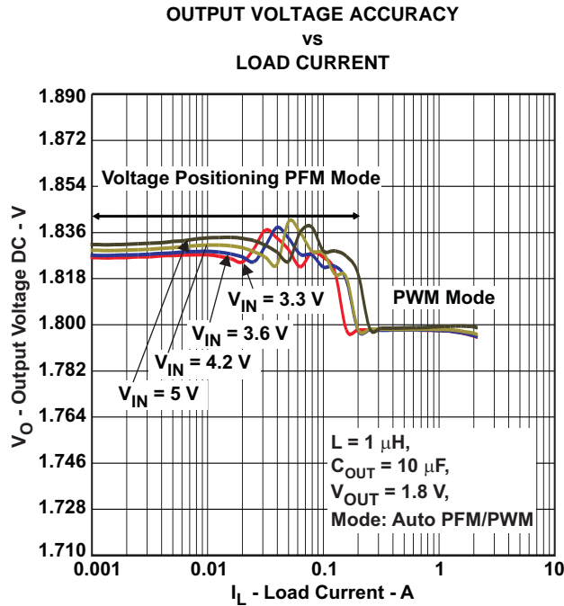
Figure 5. Auto PFM/PWM Mode
