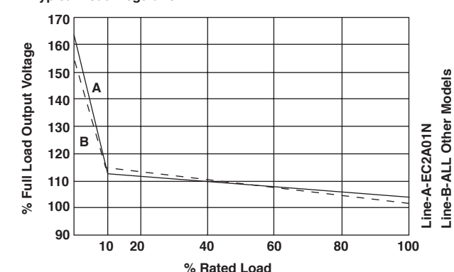
Typical Load Regulation
