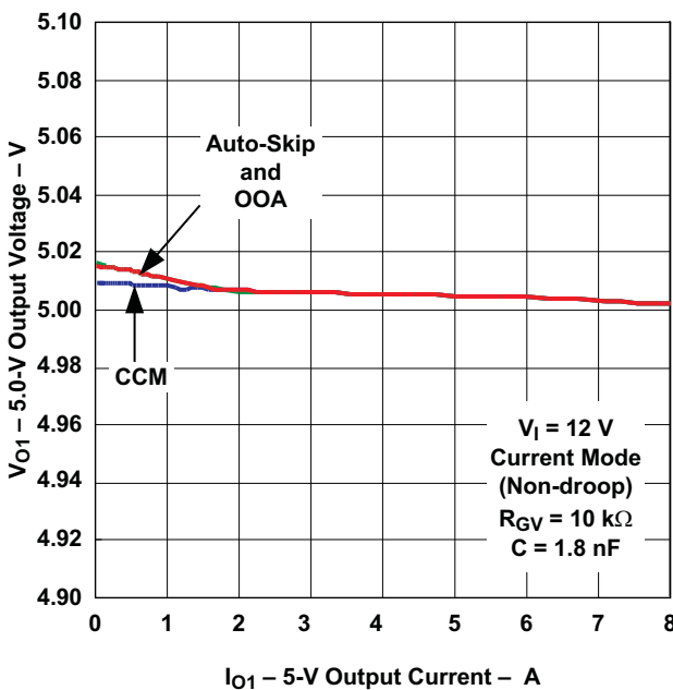
5-V OUTPUT VOLTAGE vs OUTPUT CURRENT
