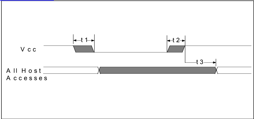
FIGURE 8 - POWER-UP TIMING
