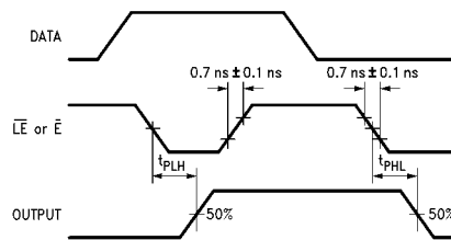
FIGURE 2. Propagation Delays
