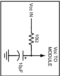
Figure 10: Supply Filter
