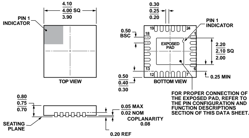
Figure 21. 24-Lead Lead Frame Chip Scale Package [LFCSP_WQ] 4 mm x 4 mm Body, Very Very Thin Quad (CP-24-1) Dimensions shown in millimeters
