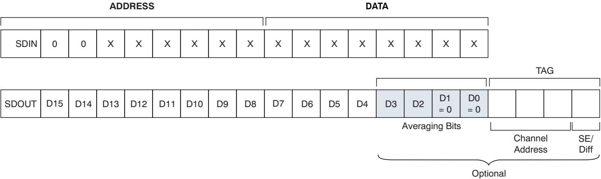
Figure 30. ADC Read
