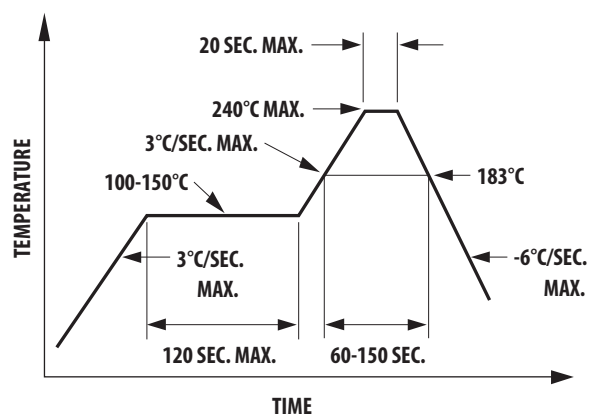
Figure 16. Recommended Lead Soldering Profile
