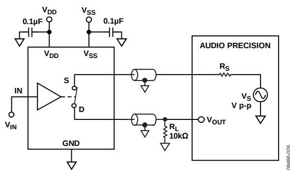
Figure 27. THD + N
