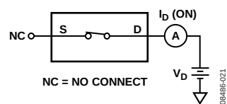
Figure 22. On Leakage
