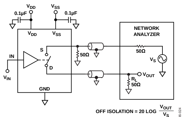
Figure 25. Off Isolation
