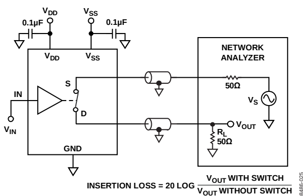
Figure 26. Bandwidth
