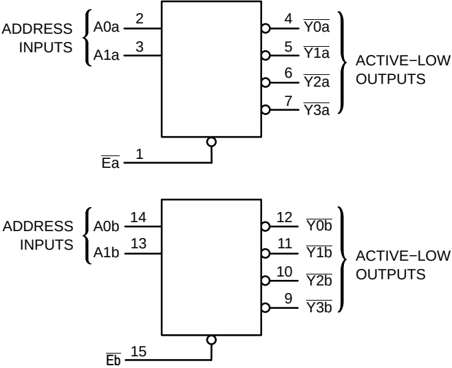
Figure 3. Logic Diagram
