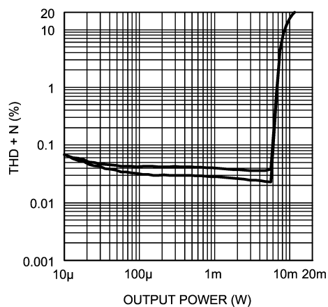
THD+N vs Output Power V_{DD} = 1.8V , R_L = 32\Omega , f = 1kHz Two channels in phase
