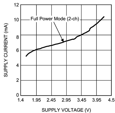
Supply Current vs Supply Voltage R_L = 16\Omega
