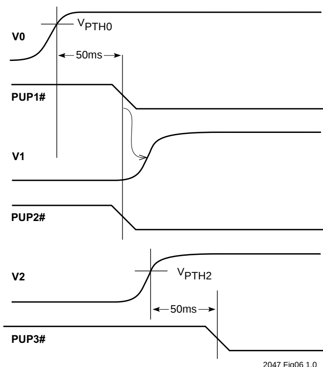
Figure 5. V_x Input and PUP# Sequence
