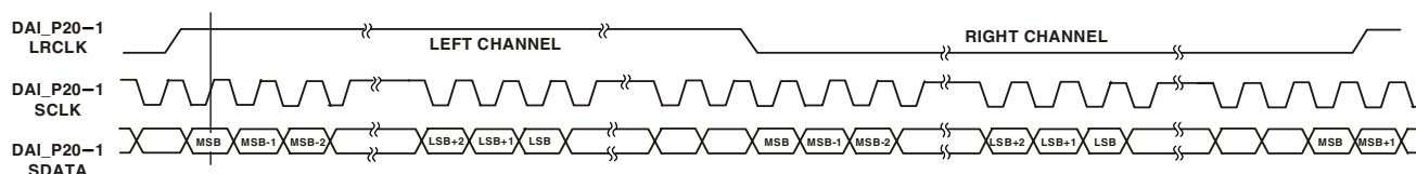
Figure 31. Left-Justified Mode
