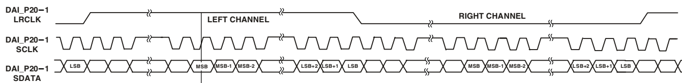
Figure 29. Right-Justified Mode
