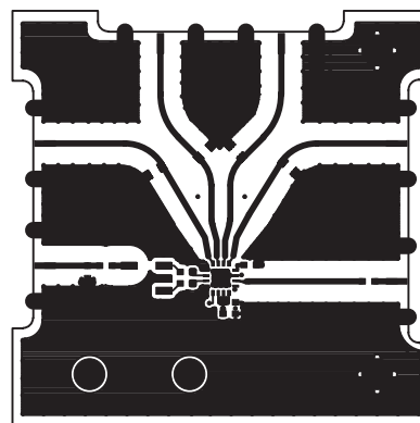
Figure 4. Component Side Layout of Evaluation Board
