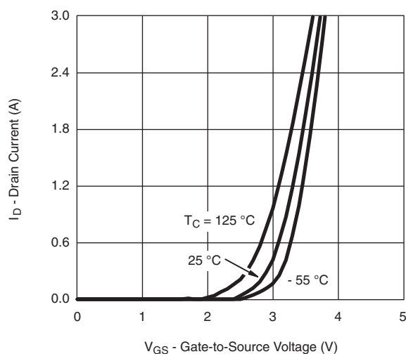
Transfer Characteristics Curves vs. Temp.
