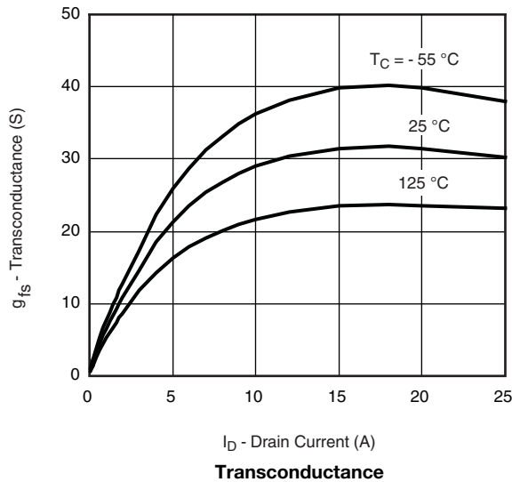
Transconductance
